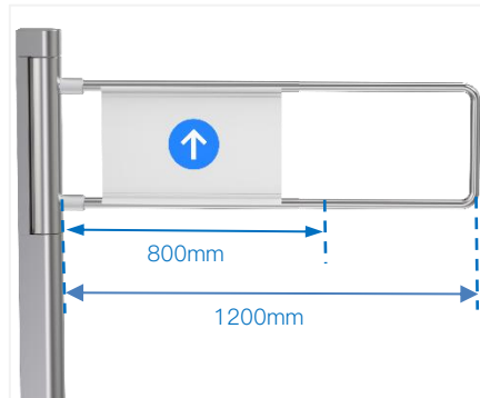
Telescopic Swing Arm
